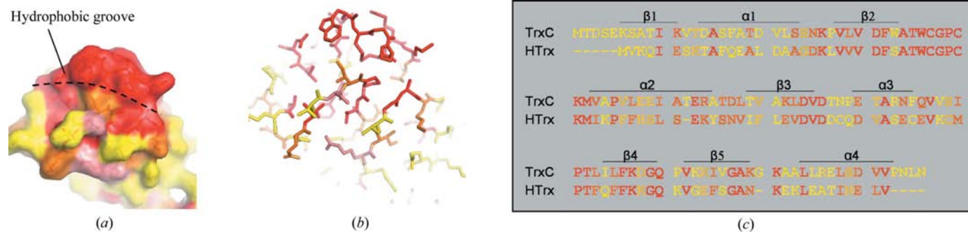
Figure 3 (a) Molecular surface and (b) ball-and-stick diagrams portraying the sequence conservation between human thioredoxin and M. tuberculosis thioredoxin C around the active-site groove, where red shows high conservation and yellow shows low conservation. (c) Sequence alignment of Mtb TrxC and human thioredoxin (hTrxC), with conserved residues coloured in the same scheme and the active site in bold.
