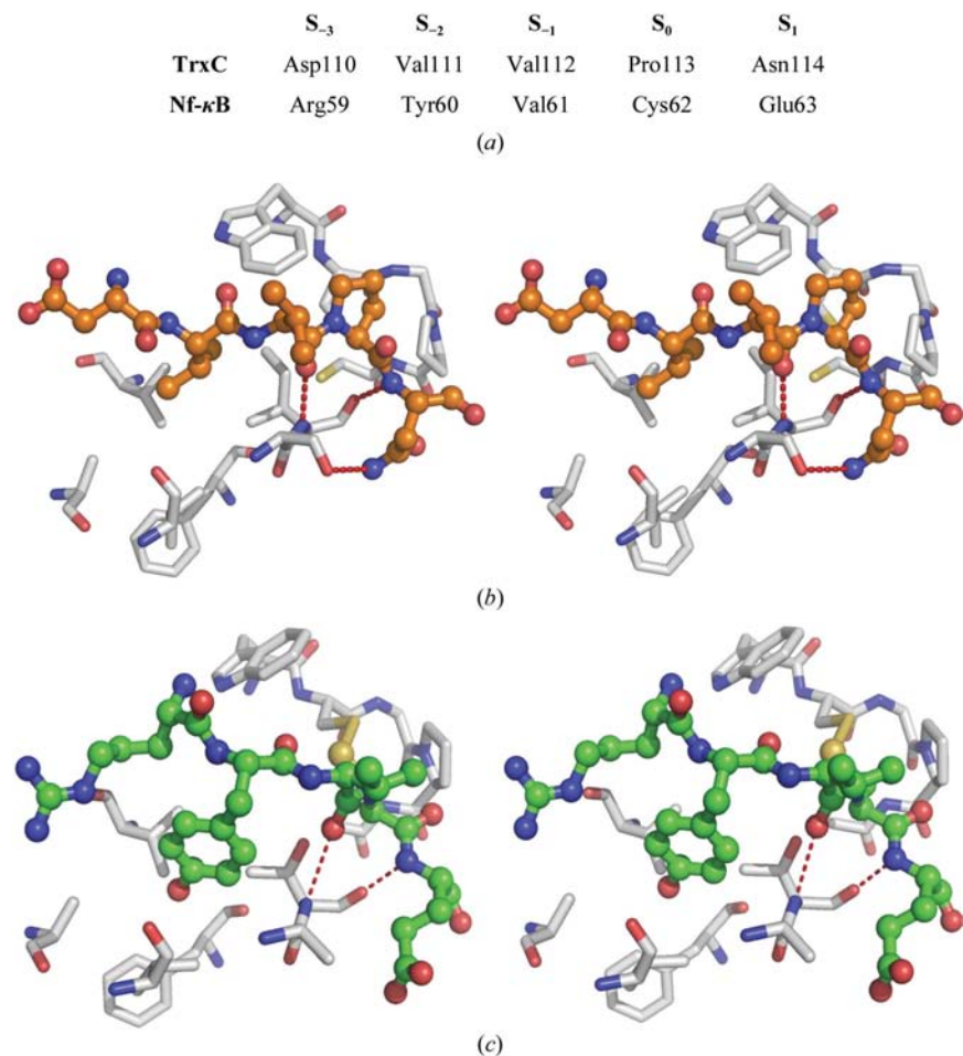
Figure 2 (a) Sequence alignment of the polypeptide tail and NF-κB residues interacting with thioredoxin. (b) Stereoviews portraying the alignment of the five C-terminal residues of the tail of Mtb TrxC and (c) five residues of the thioredoxin binding partner NF-κB from the NMR structure 1mdi (Qin et al. , 1995), resting in their respective thioredoxin active sites. The residues lining the hydrophobic pockets are also shown.
